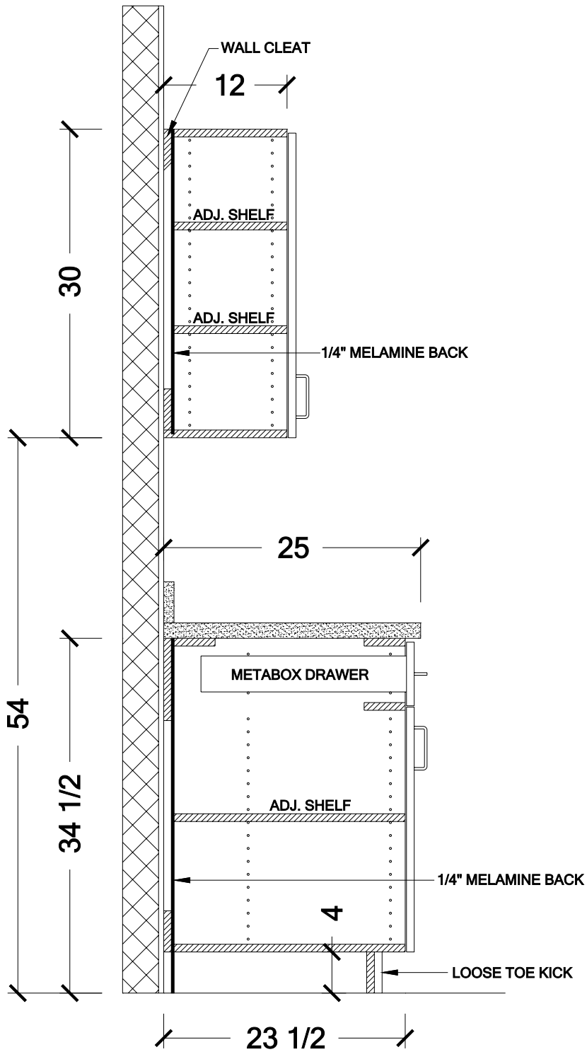
TYPICAL LAMINATE CABINET SECTION VIEW
